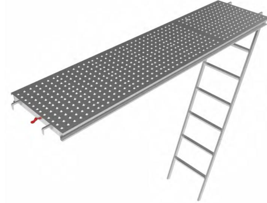
SS-US Alu Merdivenli Platform 63 SS-US Alu Ladder Deck 63
